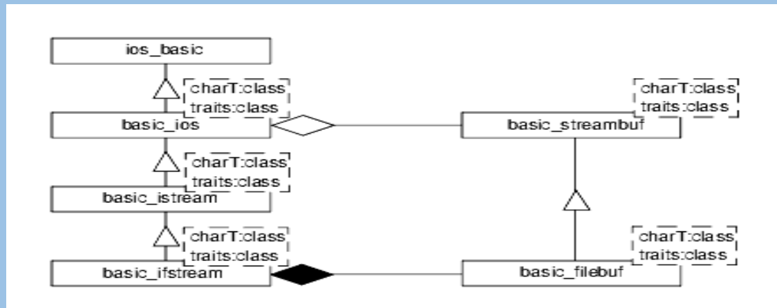
Figure 1 How an input file stream uses a file buffer
